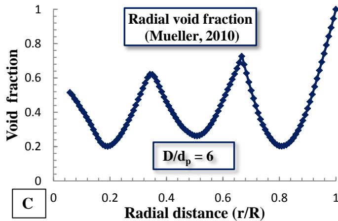
Figure 4.11: Variation in axially averaged radial void fraction model for three aspect ratios of D/d_p : A) 24, B) 12, and C) 6.
